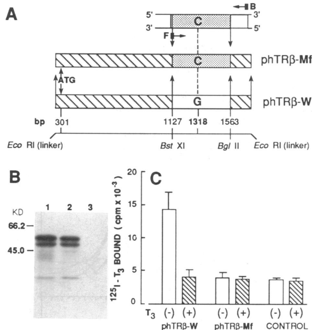
FIG. 6. Triiodothyronine binding activity of the in vitro -synthesized normal and mutant THRβ proteins. (A) Strategy of plasmid construction for in vitro translation. Filled boxes and arrows indicate the positions of primers B and F and direction of elongation used for the amplification of M13 clone. The nucleotide sequence numbers follow those of Weinberger et al. (8). (B) In vitro translation of normal and mutant THRβ . The [ 35 S]methionine-labeled products were separated by electrophoresis on 10% SDS/polyacrylamide gel that was fluorographed. Lanes: 1, phTRβ-W; 2, phTRβ-Mf, and 3, no added RNA. Protein size markers were bovine serum albumin, 66.2 kDa and ovalbumin, 45.0 kDa. (C) [ 125 I]-labeled triiodothyronine binding to in vitro translation products of normal and mutant THRβ . In vitro translation products of phTRβ-W, phTRβ-Mf, and rabbit reticulocyte lysate without mRNA (control) were incubated with 13.8 pM [ 125 I]-labeled triiodothyronine without (-) or with (+) 10 4 -fold excess unlabeled triiodothyronine. Data displayed represent the mean \pm SD of three independent duplicate experiments.
