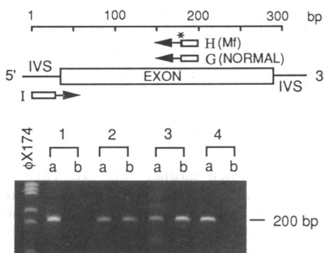
FIG. 5. Detection of normal (primer G) and mutant (primer H; Mf) THRβ alleles in genomic DNA by allele-specific amplification. DNA samples were hybridized with primers I and G (lanes a) and primers I and H (lanes b). After PCR, samples were submitted to electrophoresis in 2% GTC-agarose and stained with ethidium bromide. DNA samples 1-4 are as follows: 1, mother; 2, proband; 3, father; 4, unrelated subject with familial GRTH; \phi X174 is a size marker. IVS, intervening sequence.
