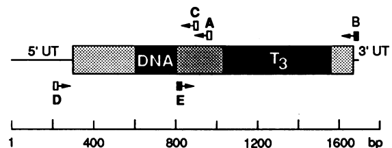
FIG. 1. Schematic representation of THRB cDNA and the cloning strategy. The shaded areas represent the coding region and its DNA and ligand-binding domains. Open boxes and filled boxes indicate primers used for amplification of 5' half and 3' half, respectively; arrows indicate positions of primers A–E and direction of elongation. UT, untranslated region; T 3 , triiodothyronine.
